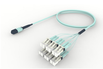
Ultra Low Loss (ULL) OM4 MPO12 (Pinned) to LC, Fiber Extension Cable Assembly, 12-Fiber, Low Smoke Zero Halogen
