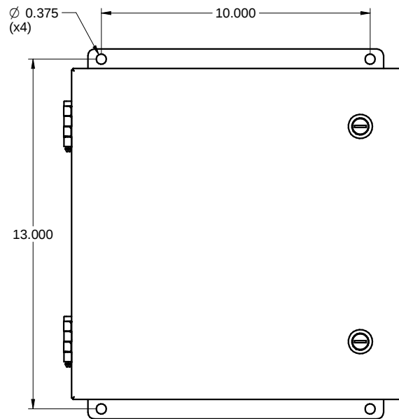
FRONT / FACE
