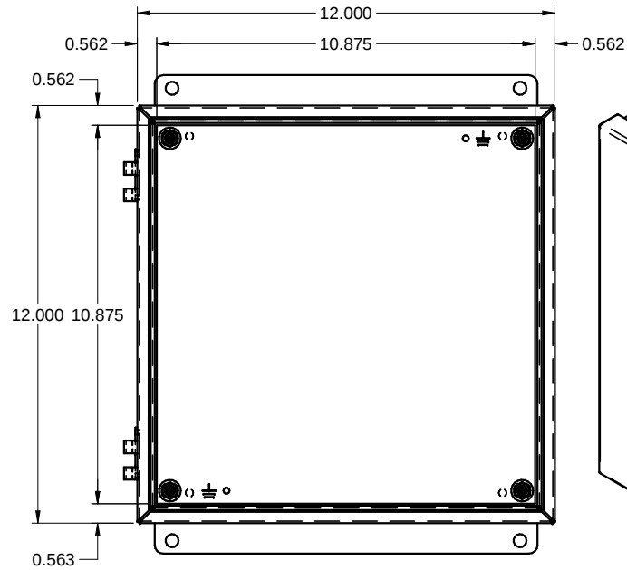
FRONT WITHOUT COVER / FACE SANS COUVERCLE
