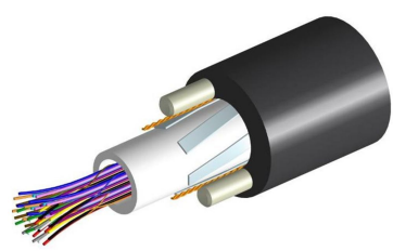
LazrSPEED® Single Jacket All-Dielectric, Gel-Filled, Outdoor Central Tube Cable
