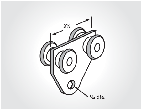
02 TR294 Can be used for series A, E and H channels only. Standard finish is electrogalvanized. Frictionless needle bearings. Design load: 1,000 lb Safety factor of 5. Wt./C 106 lb
