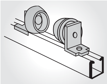
03 C728 Pipe roller (pair) Cast aluminum rollers, steel brackets. Designed for standard saddles. Order separately for each pair of rollers: two 1/2 in. x 5/16 in. hex head cap screws and two 1/2 in. channel nuts. Space to suit O.D. of pipe and wrapping. Design load: 2,350 lb Wt./C : 300 lb
