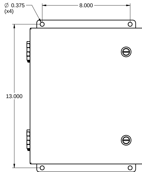
FRONT / FACE
