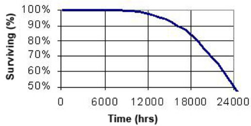
Graphs_Lumen Maintenance
