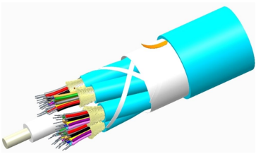
LazrSPEED® Low Smoke Zero Halogen Riser Distribution Cable, 72 fiber multi-unit with 12 fiber subunits
