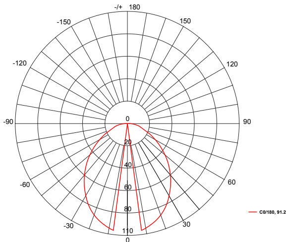
AVERAGE BEAM ANGLE (50%): 91.2 DEG
