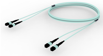
OM4 MPO (Unpinned) to MPO (Unpinned), InstaPATCH® 360 Pre-terminated Trunk Cable, 24-Fiber, Plenum
