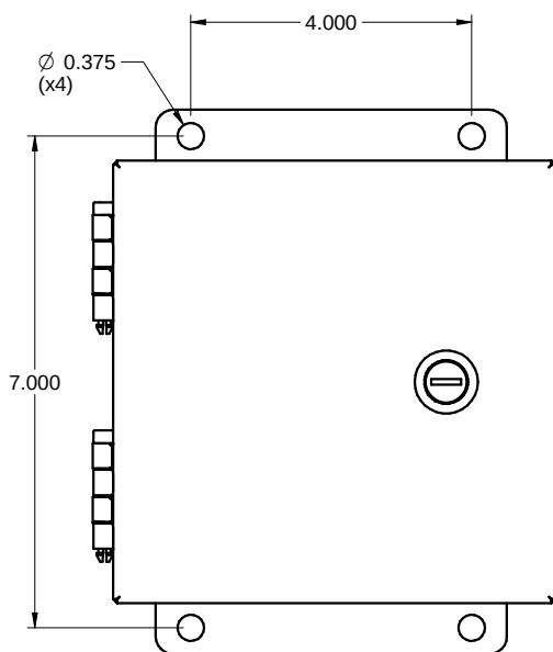
FRONT / FACE
