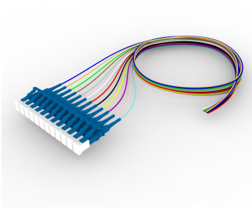
Singlemode LC to Unconnectorized, Fiber Pigtail, 0.9 mm Tight Buffer, 12-Fiber Kit Blue - Aqua (1-12)
