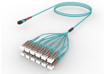
Ultra Low Loss OM4 MPO24 Pinned to LC Uniboot 24-Fiber Plenum Array Cord
