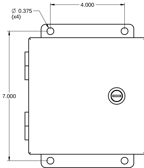
FRONT / FACE
