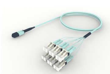
Ultra Low Loss (ULL) OM4 MPO12 (Unpinned) to LC, Fiber Extension Cable Assembly, 12-Fiber, Plenum
