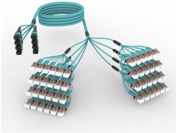
OM4 MPO (Unpinned) to LC, InstaPATCH® 360 Ruggedized Fanout Cable, 96-Fiber, Plenum
