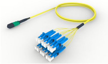
Ultra Low Loss (ULL) Singlemode MPO12 (Unpinned) to LC, Fiber Extension Cable Assembly, 12-Fiber, Low Smoke Zero Halogen
