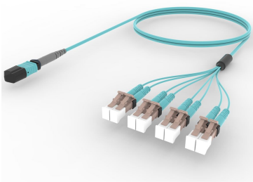
Ultra Low Loss (ULL) OM4 MPO8 (Unpinned) to LC, Fiber Extension Cable Assembly, 8-Fiber, Plenum
