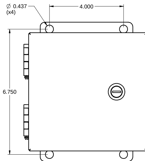
FRONT / FACE
