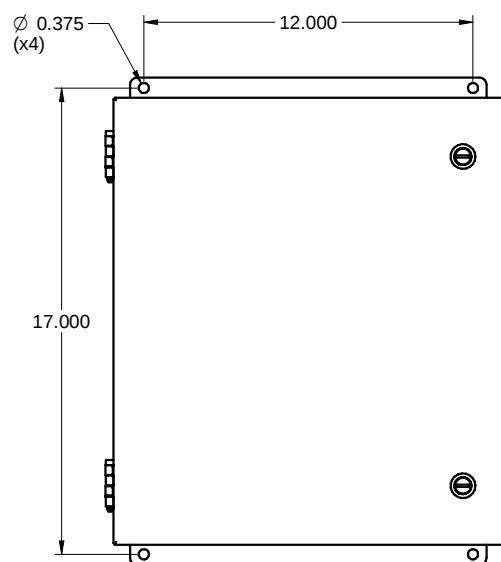
FRONT / FACE
