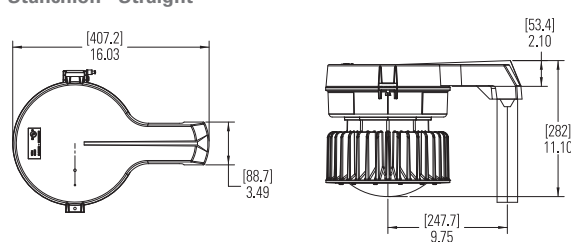
Stanchion - Straight
