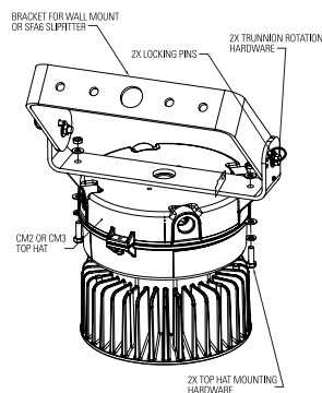
Trunnion
