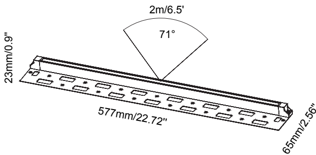
Max. Luminous intensity : 50 cd
