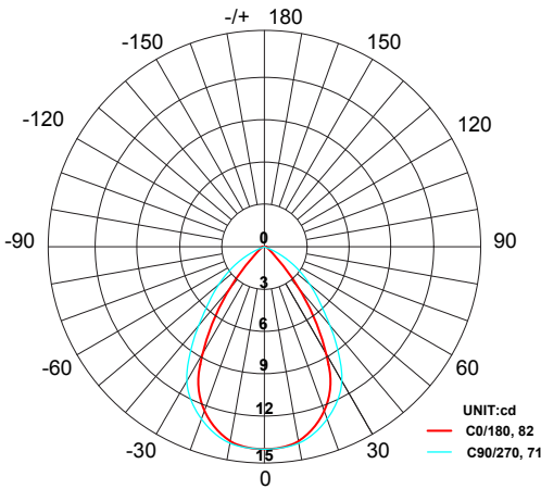
AVERAGE BEAM ANGLE (50%): 76.5 DEG
