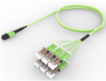
Ultra Low Loss (ULL) OM5 MPO12 (Pinned) to LC, Fiber Extension Cable Assembly, 12-Fiber, Low Smoke Zero Halogen
