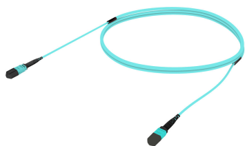
OM4 MPO12 (Pinned) to MPO12 (Pinned), Fiber Patch Cord, 12-Fiber, Method A, Plenum
