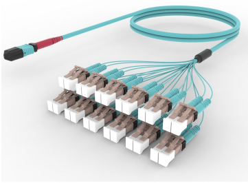
Ultra Low Loss OM4 MPO24 Unpinned to LC 24-Fiber Low Smoke Zero Halogen Array Cord
