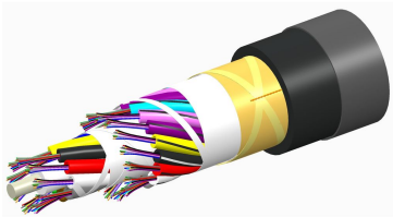
LazrSPEED® Indoor/Outdoor, Single Jacket All-Dielectric, Riser Rated, Gel-Free, Stranded Loose Tube Cable
