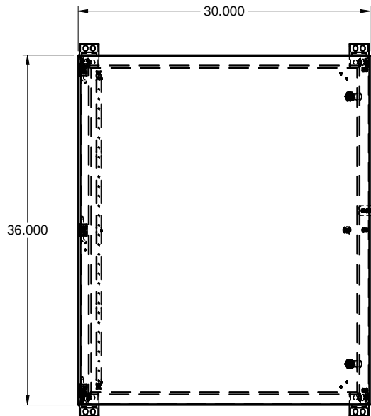
FRONT / FACE
