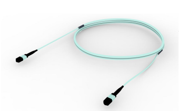
OM3 MPO (Unpinned) to MPO (Unpinned), InstaPATCH® 360 Pre-terminated Trunk Cable, 12-Fiber, Low Smoke Zero Halogen
