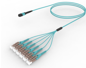
Ultra Low Loss (ULL) LazrSPEED® 550 OM4 MPO/12 (Unpinned) to LC Uniboot, 12-Fiber, Plenum
