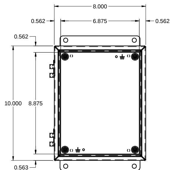
FRONT WITHOUT COVER / FACE SANS COUVERCLE
