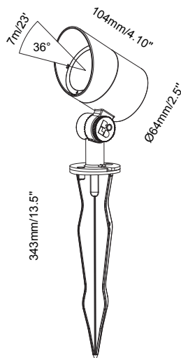
Max. Luminous intensity : 978 cd
