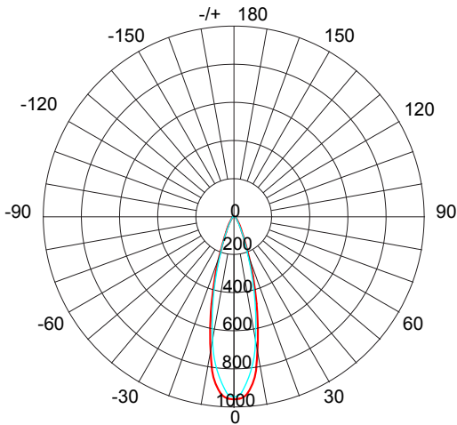
AVERAGE BEAM ANGLE (50%): 30.5 DEG
