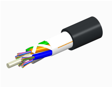
LazrSPEED® Indoor/Outdoor, Single Jacket All-Dielectric, Low Smoke Zero Halogen (LSZH), Gel-Free, Stranded Loose Tube Cable
