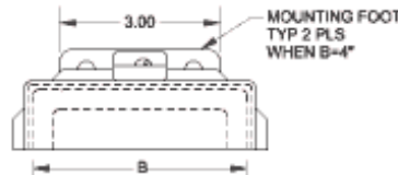
Mounting Foot Detail When B=4
