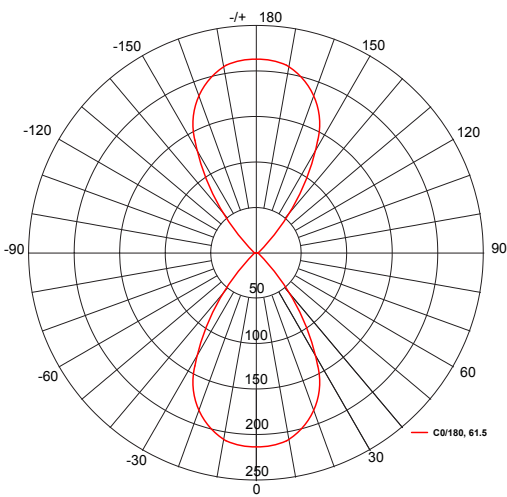
AVERAGE BEAM ANGLE (50%): 61.5 DEG
