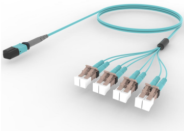
Ultra Low Loss (ULL) OM4 MPO8 (Unpinned) to LC, Fiber Extension Cable Assembly, 8-Fiber, Low Smoke Zero Halogen
