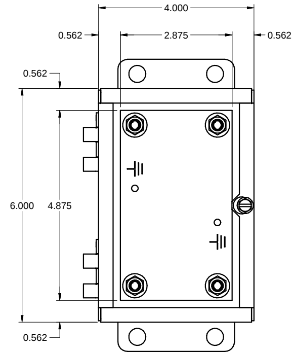
FRONT WITHOUT COVER / FACE SANS COUVERCLE
