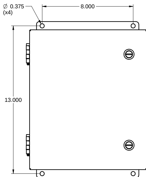
FRONT / FACE
