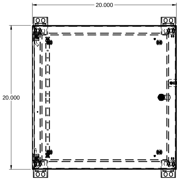
FRONT / FACE
