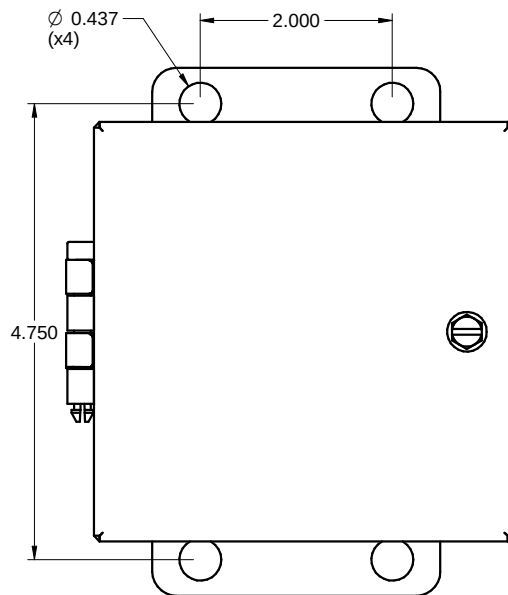
FRONT / FACE
