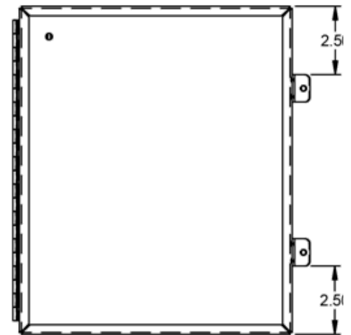
Clamp location when A = 12.0\"/>
