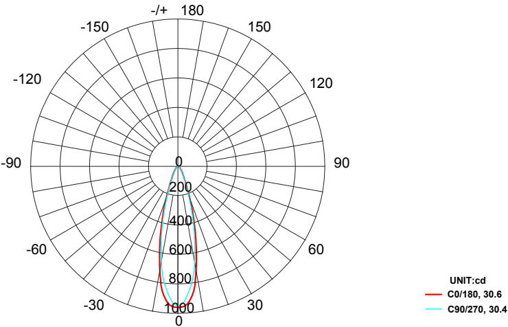
AVERAGE BEAM ANGLE (50%): 30.5 DEG
