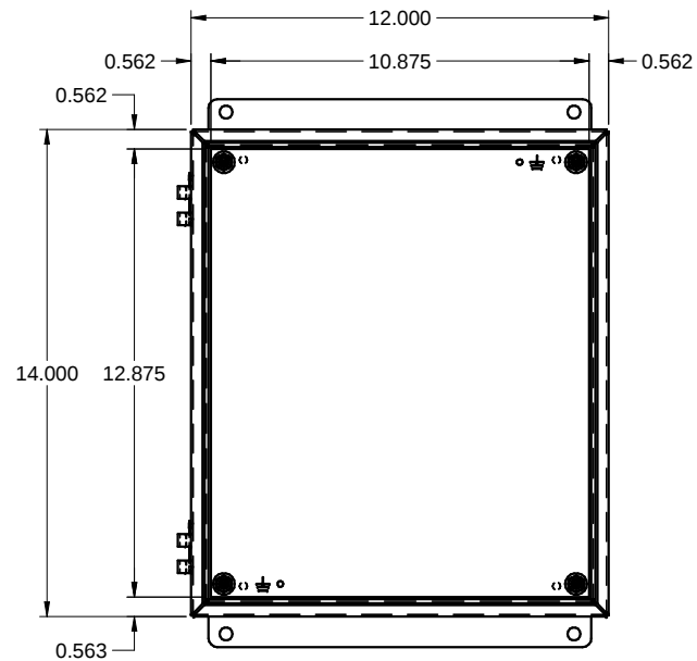
FRONT WITHOUT COVER / FACE SANS COUVERCLE
