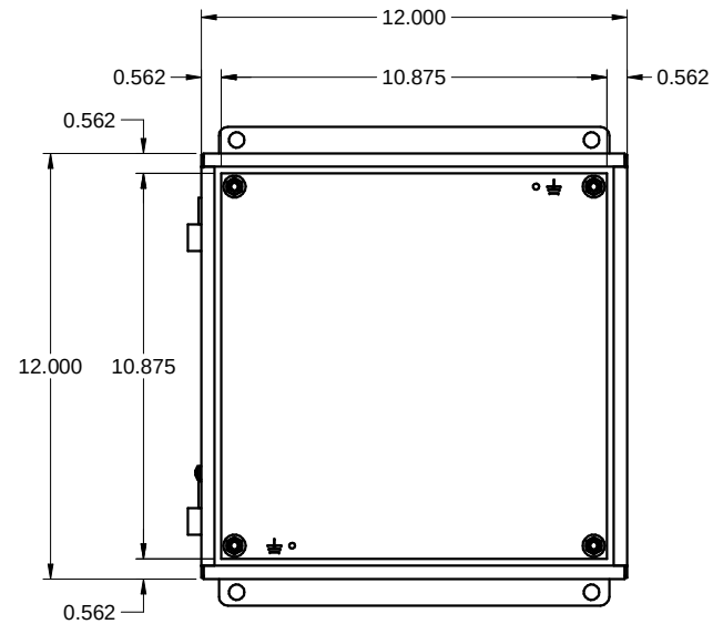
FRONT WITHOUT COVER / FACE SANS COUVERCLE
