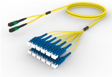
Ultra Low Loss Singlemode MPO12 Unpinned to LC Uniboot 24-Fiber Low Smoke Zero Halogen Riser Array Cord
