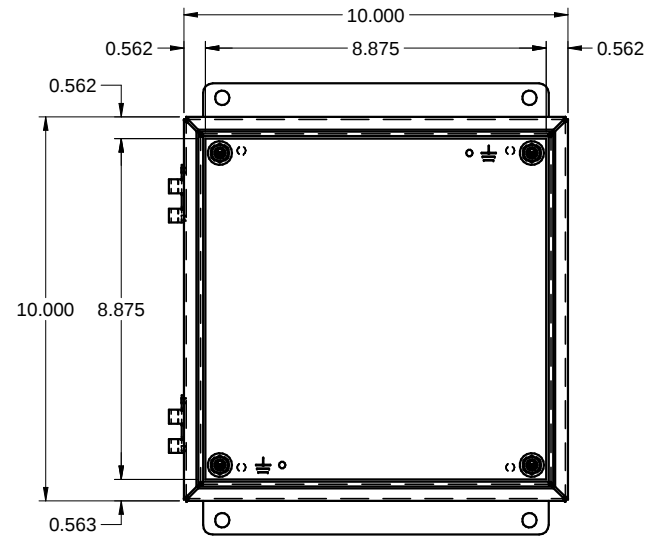
FRONT WITHOUT COVER / FACE SANS COUVERCLE
