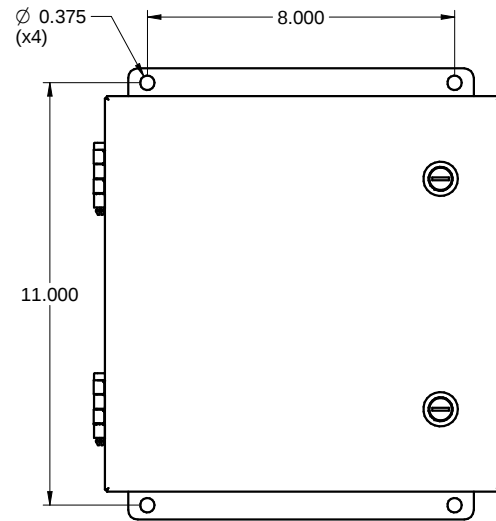
FRONT / FACE
