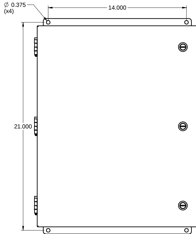
FRONT / FACE
