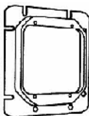
Steel Cover Plates4-11/16" Sq. - Single Device - 1" R -
