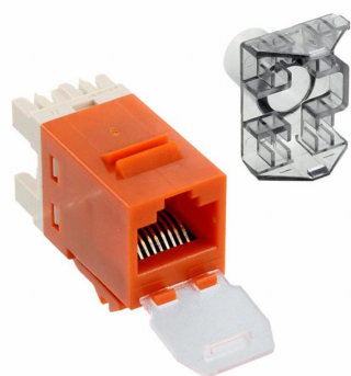
Uniprise USL Series Modular Jack, RJ45, category 6, T568A/T568B, unshielded, with dust cover, orange
