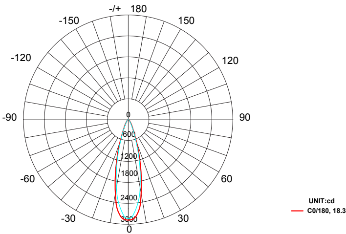
AVERAGE BEAM ANGLE (50%): 18.3DEG
