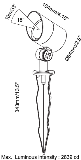
Max. Luminous intensity : 2839 cd
