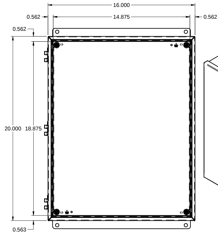
FRONT WITHOUT COVER / FACE SANS COUVERCLE
