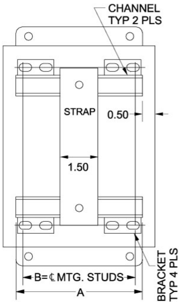
Front View
